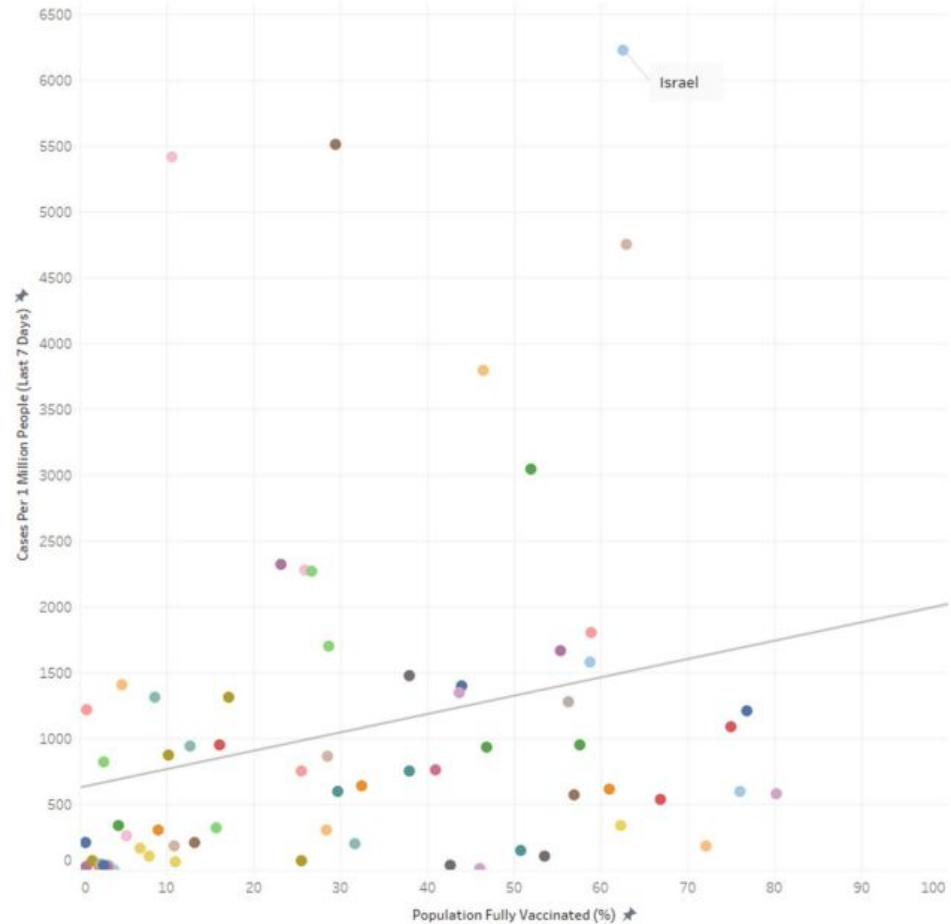
Fig. 1 Relationship between cases per 1 million people (last 7 days) and percentage of population fully vaccinated across 68 countries as of September 3, 2021 (See Table S1 for the underlying data)
